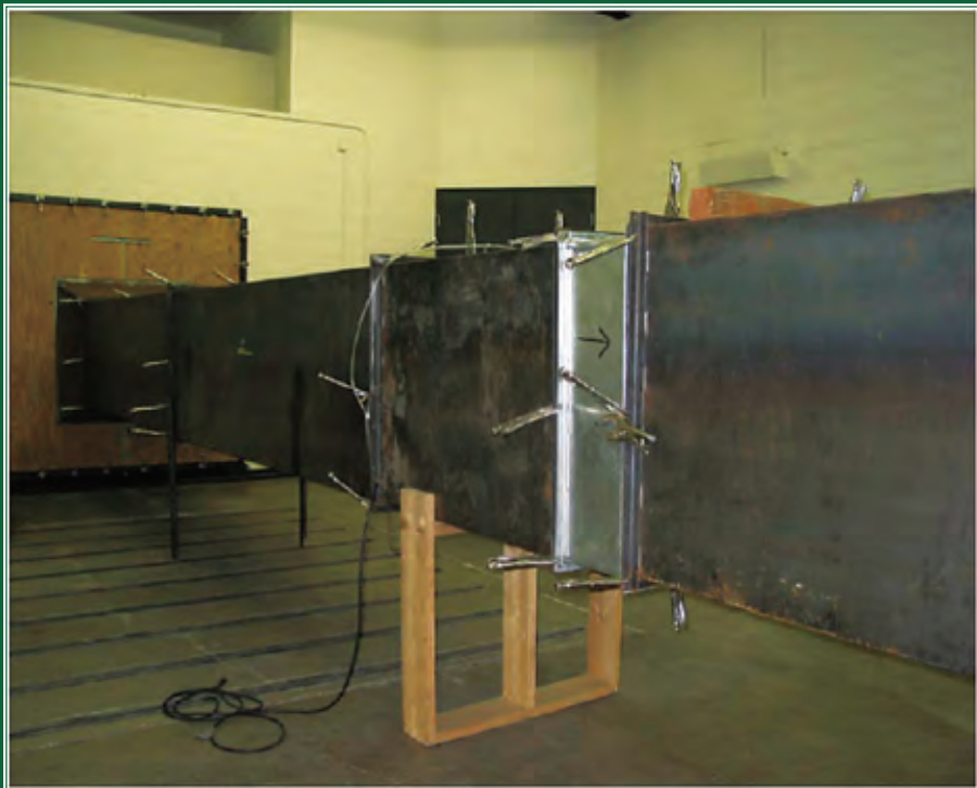
Figure5.3-Ducted Intake Test
